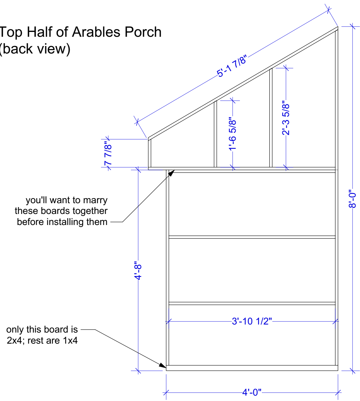
2 TD.CWArablesPorch Scale: 3/4" = 1'-0"
